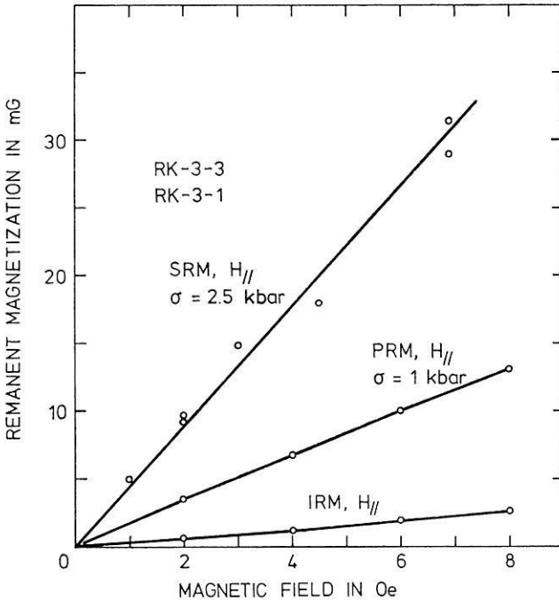
Fig. 4. Shock remanent magnetization J_r(H^+ S_1 H^e, \dots, H^+ S_n H^e) , piezo-remanent magnetization J_r(H^+ P^+ P^0 H^e) and isothermal remanent magnetization as functions of the applied magnetic field. For the SRM final steady state values obtained after several impacts are plotted
