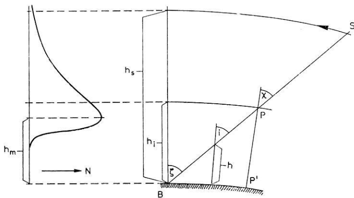
Fig. 1. Geometry receiving station ( B ) — position of the satellite ( S ) — ionospheric point ( P ) — subionospheric point ( P' ). ( b_i : mean ionospheric height, b_m : height of the maximum of the electron density, b_s : height of the satellite)
