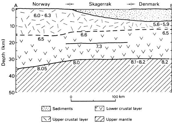
Fig. 2. Crustal structure along profile AB (Fig. 1) from seismic investigations. Results from lines within a distance of \pm 50 km are projected on to the profile. The figures indicate P -wave velocities ( \text{km s}^{-1} )
