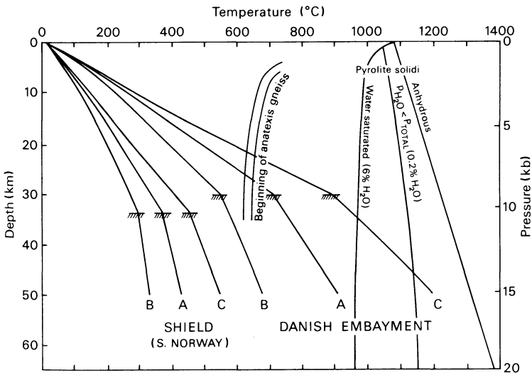
Fig. 7. The average temperature-depth functions of Table 2 in relation to the pyrolite solidi from Green (1973) and the zone of beginning of anatexis from Winkler (1974). The position of the Moho is indicated (-----)
