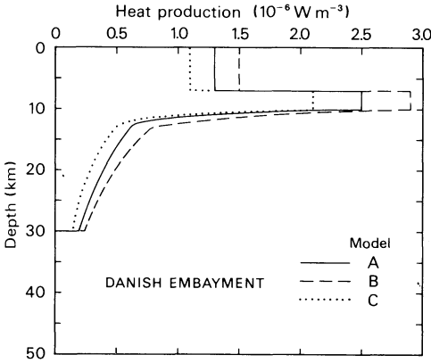
Fig. 5. Assumed heat production models of the Danish Embayment (central part)
