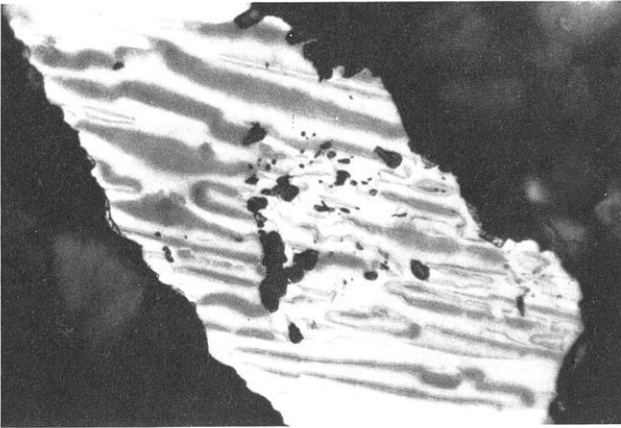
Fig. 8. Large multidomain grain with lamellae-shaped domains. The cluster of nonmagnetic inclusions within the ore grain produces extremely small domains with presumably pseudo-single-domain behaviour. The diameter of the figure is 120 \mu\text{m}
