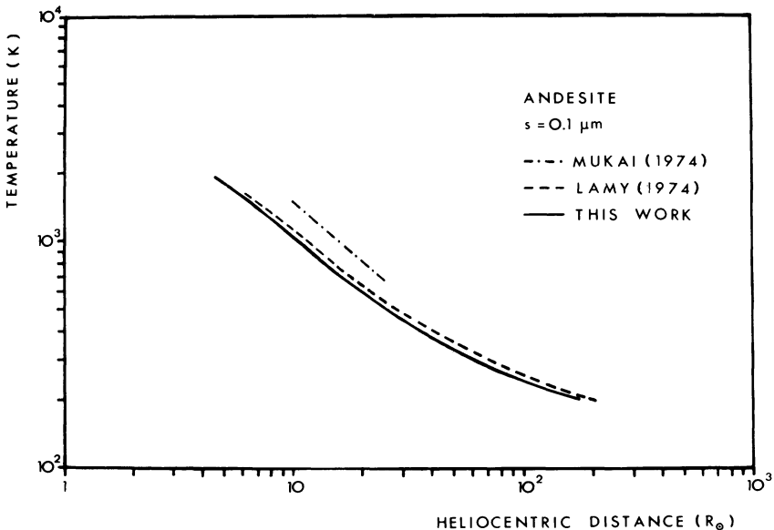
Fig. 6. Temperature of an andesite grain as a function of heliocentric distance. The dashed and dashed dotted lines give the results published by Lamy (1974) and Mukai (1974), respectively, for the same particle.
