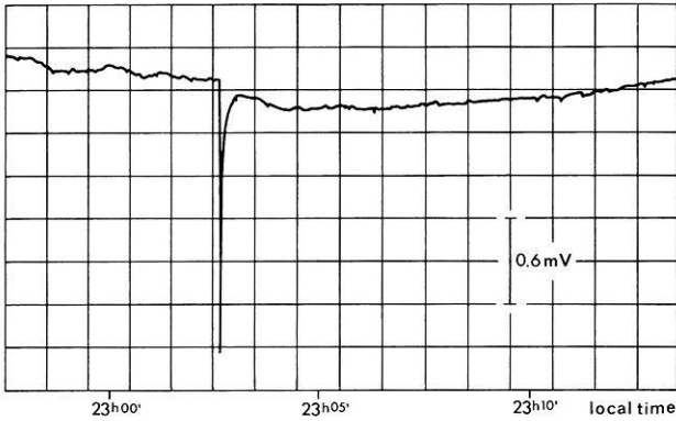
Fig. 5. Similar to Figure 3, but AB = 1250 km, MN direction parallel to AB direction. A current of 2950 amp was switched off within 20 ms. Station south of Fort Victoria
