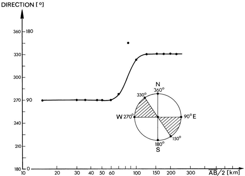
Fig. 8. Direction of the electric field as a function of \overline{AB}/2 at the sounding station INY II (cf. Fig. 9). The AB direction varied within \pm 4 degrees from the NS direction ( 0^\circ, 180^\circ , respectively)
