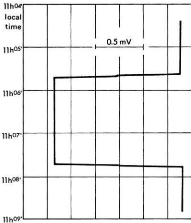
Fig. 3. Reproduction of a typical record of the potential difference \Delta V as a function of time for a current-electrode spacing \overline{AB} = 30 km and a sounding-electrode spacing \overline{MN} = 100 m. The direction of the sounding dipole MN is N 60^\circ E , applied current \pm 60 amp, station Umtali farm (FARM) (cf. Fig. 9). Local time = GMT + 2 h
