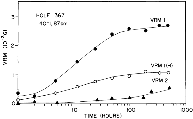
Fig. 8. Acquisition of VRM in presence of NRM (VRM 1) and after AF demagnetization (VRM 2) in a DSDP basalt sample from a site in the Jurassic Quiet Zone in the eastern North Atlantic. VRM 1 (H) represents the change in remanence in the plane perpendicular to the applied field of 1 Oe
