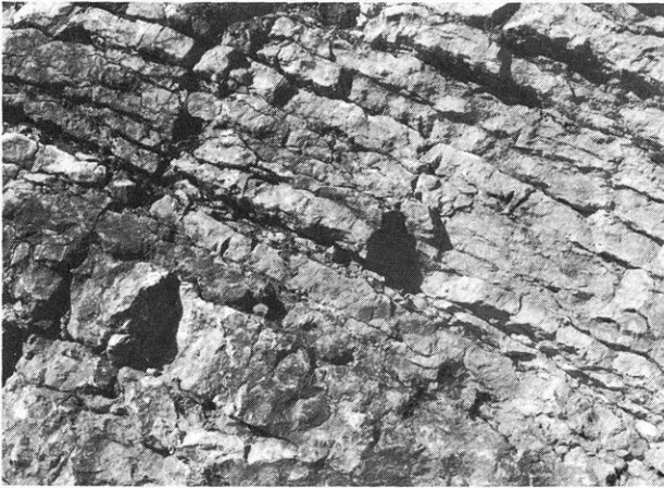
Fig. 4. Typical outcrop of red nodular Adneter Kalk. Königsbachtal (loc. No. 6)
