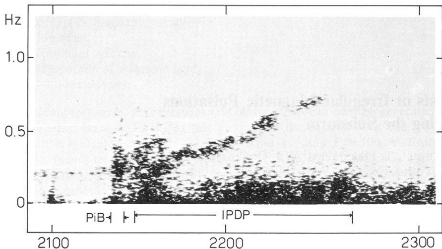
Fig. 1. Dynamic spectrum of magnetic pulsations at Sodankylä on October 5, 1974, illustrating the appearance of PiB and IPDP events
