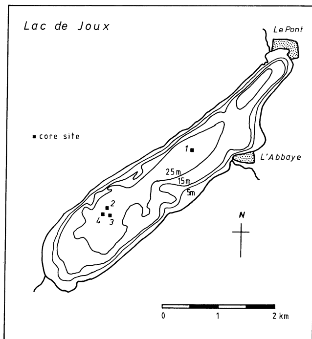
Fig. 1. Sketch map of Lac de Joux ( 46.6^{\circ}N , 6.3^{\circ}E ) showing coring sites. Contours show water depths in the lake
