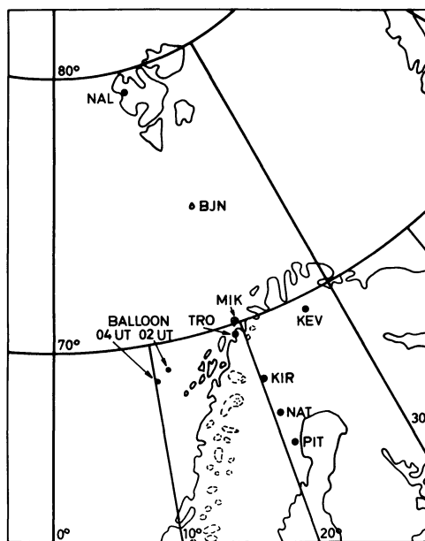
Fig. 1. Map showing the location of the observing stations and the balloon
