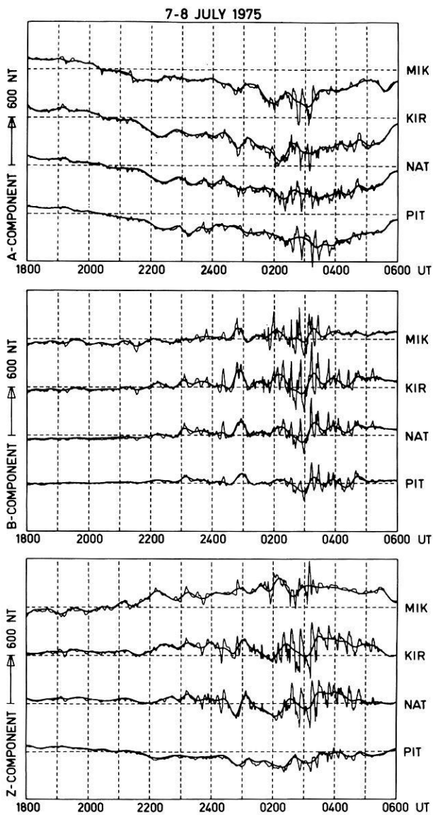
Fig. 4. Münster magnetograms, with low pass filtered ( T > 30 min) data superimposed
