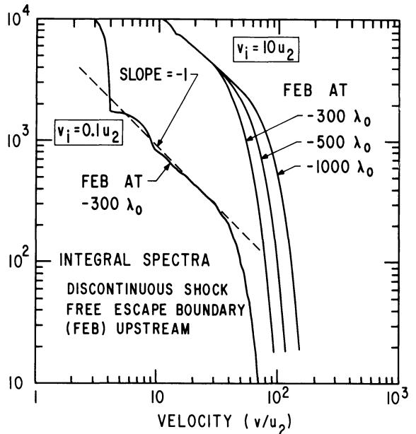
Fig. 2. Integral velocity spectra for a discontinuous shock with v_i=0.1 and 10u_2 . The dashed line shows the expected slope obtained from the diffusion approximation. The position of the free escape boundary is measured in units of \lambda_0 , the mean free path of a particle with A/Z=1 , v=u_2 , and \rho=\rho_2 .
