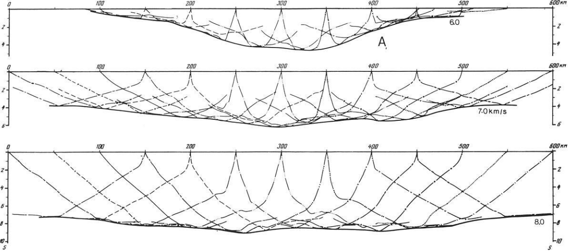
Fig. 2. a Crustal model with a graben-like depression and the calculated travel-time curves from a number of shot points. b Reduced travel-time curves and their envelopes (6.0, 7.0, 8.0 km/s). c Reduced travel-time curves and their envelopes (7.0 and 8.0 km/s) after having applied the time correction based on the topography of the isoline v = 6 km/s. d Comparison of different interpolation results with the original model. 1. boundaries based on one-dimensional solutions for each shot point; 2. derived from the system of reduced travel-time curves
