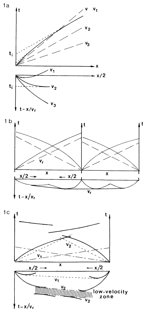
Fig. 1. a Reduced and transformed travel-time curves t - x/v_r with different reduction velocities v_1, v_2, v_3 for one shot point. b Construction of a velocity-isoline v_r based on travel-time curves from a number of shot points. c Detection of a low-velocity layer in the reduced time section
