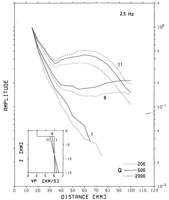
Fig. 12. Amplitude-distance curves for models PG1, PG6 and PG11 (see inset and Table 1) for Q=500 , continuous lines, Q=200 , dotted lines and Q=2000 (dashed line for model PG11)
