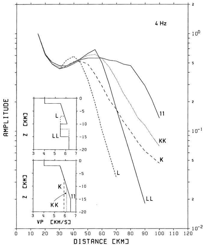
Fig. 8. Amplitude-distance curves for models PG11, PG11K, PG11KK with variable gradient zone thickness ( continuous, dashed and dotted lines , respectively in the lower inset ) and PG11L and PG11LL with low-velocity layer at different depths ( dashed and continuous lines , respectively, in the upper inset ) computed for a frequency of 4 Hz
