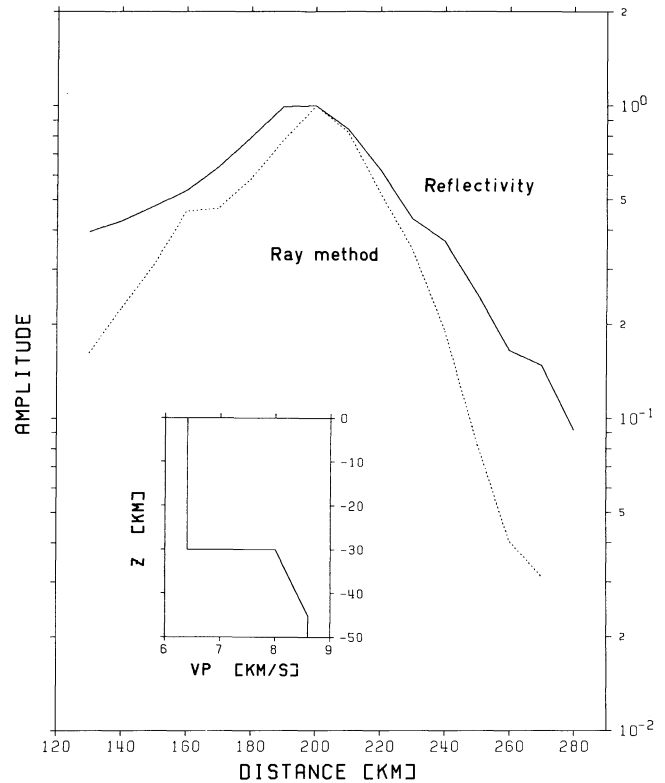
Fig. 2. Amplitude-distance curves (peak-peak) of P_n phase for model EC4 (Červený, 1979) computed using reflectivity (continuous line) and using ray-method (dotted line)
