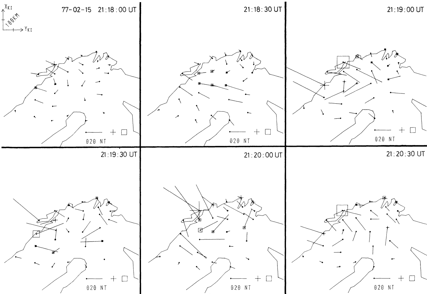
Fig. 11. Spatial distribution of equivalent current vectors of the high-pass filtered records for six successive times on 15 February 1977. The current vectors have their origin where the corresponding magnetic disturbances have been recorded; squares and crosses denote negative and positive Z perturbations, respectively
