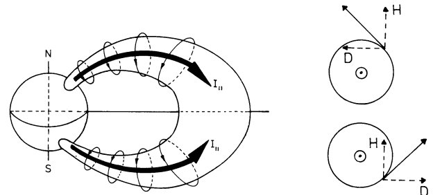
Fig. 13. Schematic view of the generation of odd-mode standing oscillations in the magnetospheric magnetic field by line-type upward field-aligned currents. In the right part the magnetic field generated in the magnetosphere by an upward field-aligned current in the northern and southern hemisphere is shown schematically (after Raspopov, 1976)
