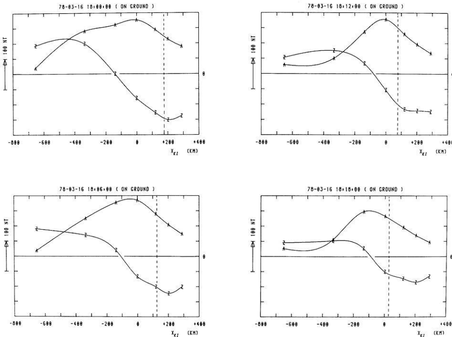
Fig. 5. Latitudinal profiles of the magnetic horizontal components parallel to the x_{KI} axis (A) and of the vertical components (Z) observed at 1800, 1806, 1812 and 1818 UT on profile 4 of the SMA. The letters denote the A and Z profiles and simultaneously give the observed values. The dashed vertical lines give the positions of the most equatorward discrete auroral arc
