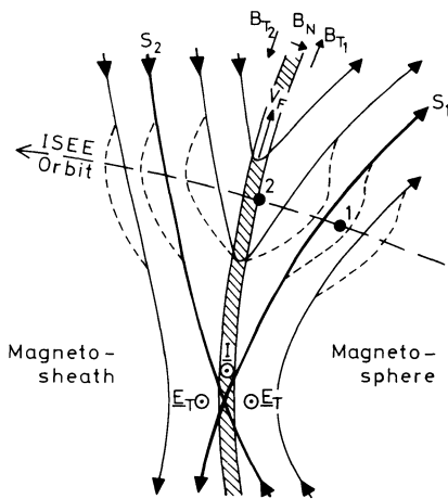
Fig. 1. Meridian cross-section of the dayside magnetopause illustrating the signatures of steady subsolar reconnection for antiparallel external and internal magnetic fields. The field lines are shown as solid lines, with the dashed lines denoting the field distortions which may occur following a short pulse of stronger reconnection which erodes extra flux
