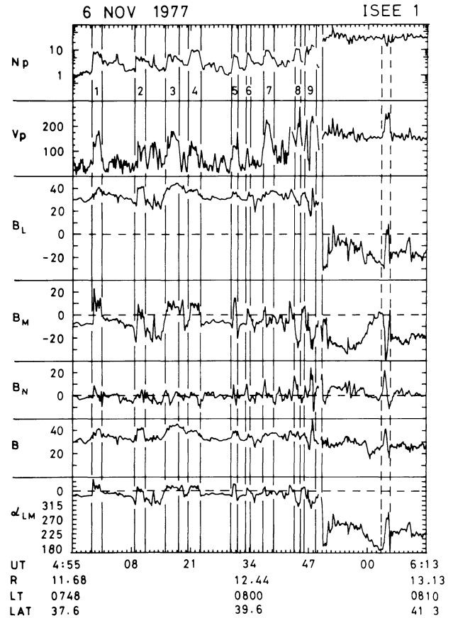
Fig. 5. ISEE 1 plasma and magnetometer recordings for the 6 November 1977 outbound crossing of the low latitude boundary layer and magnetopause. With the exception of \alpha_{LM} , the field angle in the LM plane, the plotted parameters are the same as described previously. The main intervals (or "pulses") of flowing boundary layer plasma are marked by vertical lines and numbered near the top of the diagram. A magnetosheath FTE is bracketed by the dashed guidelines at \sim 06:04 UT
