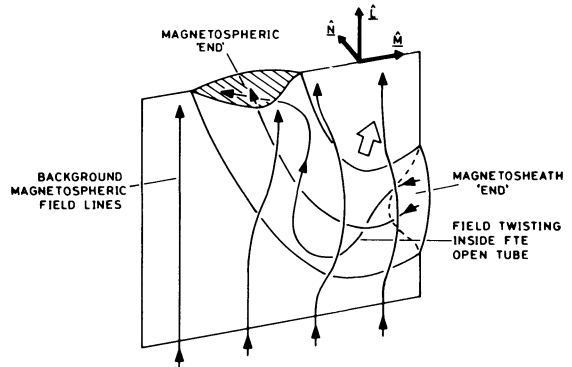
Fig. 6. Sketch of a tailward and northward propagating FTE observed from inside the magnetosphere. The field within the open tube is shown twisted as implied by the observed B_N perturbations. It is suggested that these "internal" FTEs may correspond to the BL "pulses" reported, for example, by Scokpe et al. (1981)
