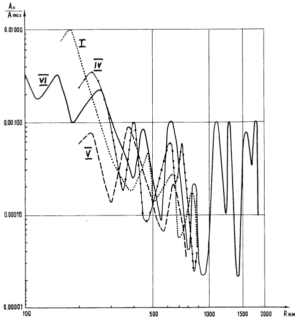
Fig. 7. Normalized amplitude curves of the mantle reflections for the profiles I, IV, V, VI
