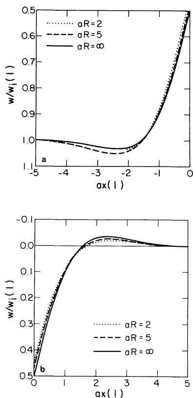
Fig. 2a and b. Normalized vertical displacement w/w_i as a function of non-dimensional distance ax from the edge of the disk load for different non-dimensional radii aR and a points below the load or b beside the load. w_i denotes the displacement for local compensation
