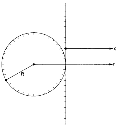
Fig. 1. Straight-edged axisymmetric load and its two-dimensional approximation
