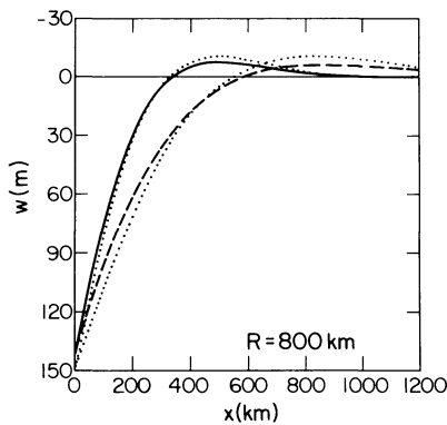
Fig. 4. Vertical displacement w for a disk radius of R = 800 km as a function of distance from the load edge for h = 100 km or aR = 5.46 (solid) and h = 200 km or aR = 3.24 (dashed). The dotted lines delineate the appropriate two-dimensional solutions
