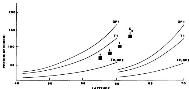
Fig. 1. Some typical eigenperiods for standing waves in the latitude range 45^\circ – 70^\circ with the plasmopause located at 60^\circ ( L=4 ). GP1 and T1 are the fundamental guided poloidal and toroidal eigenperiods; GP2 and T2 are the second-harmonic guided poloidal and toroidal eigenperiods. The squares represent the estimated periods of surface waves at the plasmopause for four different positions of the plasmopause corresponding to different levels of magnetic activity
