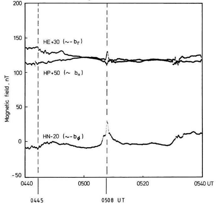
Fig. 13. GOES 2 magnetic observations for the time interval 0440–0540 UT on August 31, 1978; HE corresponds to -b_r , HN to -b_\phi , and HP to b_{||} . The numbers at the component code give values which have to be subtracted from the scale value, i.e. HP + 50 with a value 120 nT is actually 70 nT
