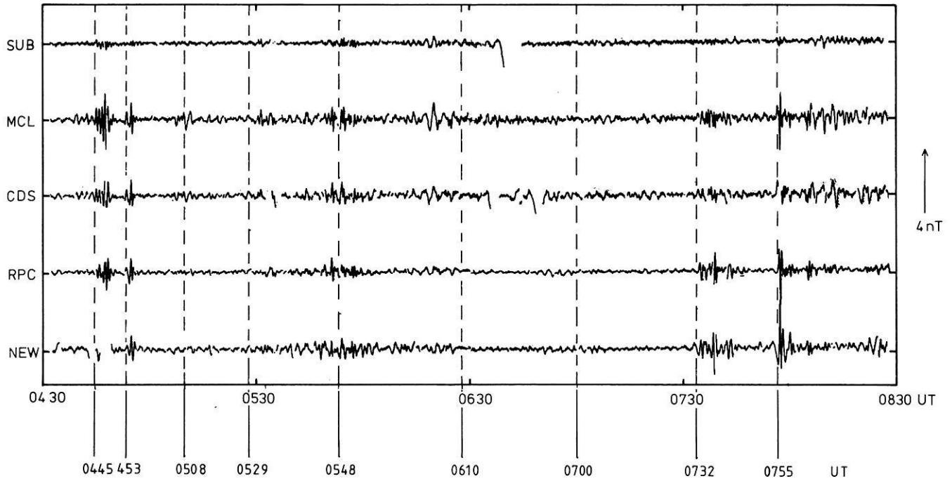
Fig. 12. Bandpass-filtered ( 50 \text{ s} < T < 150 \text{ s} ) data of the NS component of the geomagnetic disturbance field at the stations of the AFGL mid-latitude chain
