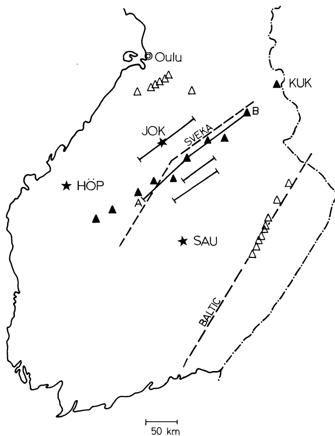
Fig. 6. Deep EM data in Finland (data set F). Solid triangles : MTS points (Ádám et al. 1982, Korja 1983). Open triangles : MTS points under analysis. Stars : MV stations of data set J3 (IMS/Jones, 1983). A-B: main scalar AMT profile (cf. Fig. 7). —: additional AMT profiles. ----: DSS profiles, SVEKA and BALTIC
