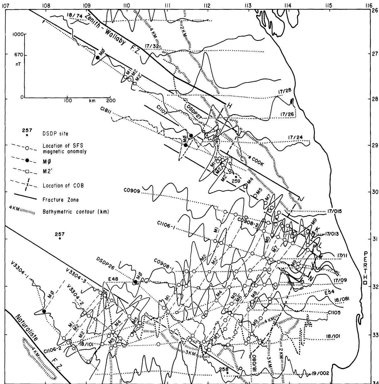
Fig. 5. Selected ships' tracks and magnetic profiles for the southern area. New profile for segment IJ from Cook; rest of profiles compiled from Markl (1974a, b; 1978a, b), Davies et al. (1973), Veevers et al. (1974), Hawkins et al. (1965) and BMR Margins Survey. Magnetic-anomaly determinations south of latitude 31°S slightly amended from Markl; north of 31°S, in segments J to M, amended after Larson et al. (1978). Determinations in IJ and of COB anomaly by us
