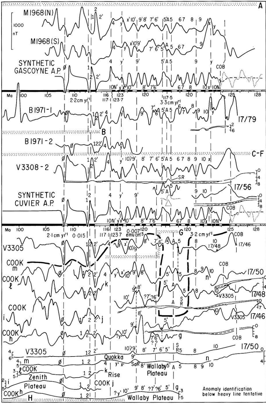
Fig. 4. a Selected magnetic, seismic and bathymetric profiles, located in Fig. 3, projected on an azimuth of 302°. Fracture zones A–H shown by stippled lines . Block model of M-series (Larson and Hilde, 1975) with normal polarity in black , reversed polarity clear —note that ages are expressed in the old K/Ar decay constants for direct comparison with previous work — and synthetic magnetic anomalies, involving reflection of blocks about axis (A), after Larson (1977), Larson et al. (1979) and Johnson et al. (1980) for the Cuvier Abyssal Plain, extended by us to the Gascoyne Abyssal Plain and tentatively to the Wallaby/Quokka region, distinguished from area of established anomalies by a heavy broken line . Model parameters not shown on the figure are: model source is 5.5–6.0 km below sea level and trend is 030°; present-day magnetic field parameters are inclination 55° up and declination 2° west. Remanent-magnetization parameters are inclination 55° up and declination 40° west. Remanent-magnetization intensity is expressed in old units of emu/cm 3 (=10 -3 A/m) to provide direct comparison with previous work. The positive anomaly at 122.4 Ma is labelled x , and the negative anomaly at 122.7 Ma, y . Lines through modelled anomalies afford direct comparison with observed anomalies; note offset of M7', A and M8 on V3305 and southward. SR = Sonne Ridge, whose magnetic anomaly is modelled by adding the magnetic response of a ridge with intensity 0.00075 emu/cm 3 to the block model ( dotted line ). Sa R – Sonja Ridge. The COB is located at 123.7 Ma in the Gascoyne Abyssal Plain and at 124.9 Ma in the Cuvier Abyssal Plain. The block model is extended ( dotted blocks ) past 125 Ma, and its magnetic profile shown by a dotted line . Track crossings are shown by triangles . Depths of seismic profiles in seconds of reflection time. Bathymetric profiles (km) of tracks across Zenith Plateau, Quokka Rise and Wallaby Plateau are concentrated at the bottom. Scales: 150 km are equivalent to 1000 nT. b Block model and synthetic magnetic anomalies in segment CE, extended from determinations by Larson (1977). Depth of seismic profiles in seconds of reflection time. Model parameters not indicated in the figure are as in Fig. 4a
