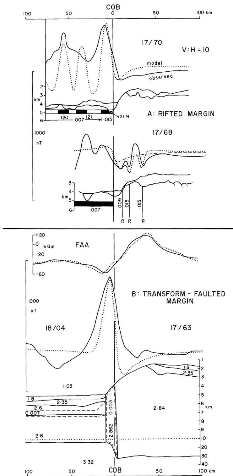
Fig. 10. A, models of the COB anomaly along the rifted margin on the western side of the Exmouth Plateau (17/70 and 17/68) projected on an azimuth of 302° and B, across the transform-faulted southern side (18/04-17/63) projected on an azimuth of 032°. The simple COB anomaly in 17/70 at the rifted margin is modelled (with the field parameters as given in Fig. 4) by modifying the magnetization of the oldest oceanic block of the seafloor-spreading sequence so that it has double the remanent-magnetization intensity of the others (as shown) or double the thickness. In 17/68, also at the rifted margin, a simple oceanic magnetic block of uniform intensity against non-magnetic continental crust produces the anomaly shown by the dotted line on the oceanic side and the broken line on the continental side; the addition of magnetic dykes of reversed polarity (R) near the edge of the continent simulates the complete set of anomalies. In 18/04-17/63, at the transform-faulted margin, a dense (2.862 t/m 3 ) vertical body at the COB is required to account for the free-air gravity anomaly (FAA) (Willcox, 1977; Roots et al. 1979; Exon and Willcox, 1980), implying a vertical body emplaced along the Cape Range FZ, interpreted from seismic diffractions at the foot of the slope (Exon and Willcox, 1980). Vertical exaggeration is x 10 above 10 km depth, x 1 below. Other densities from refraction velocities found by Larson et al. (1979). The magnetic anomaly is modelled by two bodies, outlined by broken lines : (1) part of oceanic layer 2 (density = 2.6 t/m 3 , remanent-magnetization intensity = 0.007 emu/cm 3 ) and (2) a nearly vertical body (density = 2.862 t/m 3 , intensity = 0.003 emu/cm 3 ). Other parameters as in Fig. 4. The width of the model anomaly is less than that observed, but is close to that of the other crossings of the Cape Range Fracture Zone
