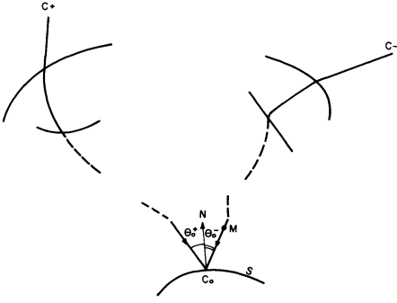
Fig. 1. Ray path for considered model (a 2-D ray scheme is shown for simplicity). C^+ is the point of emission; C^- is the point of observation; S is the scattering surface; \theta_0^+ and \theta_0^- are angles of incidence in positive and negative directions; C_0 is the specular point
