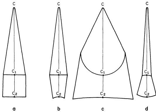
Fig. 7a-d. Examples of the cross-sections of the Fresnel volumes in E_{\parallel} for some of the models shown in Fig. 6: a Cross-section for model with R_1^{(1)}(0)=R_1^{(2)}(0)=\infty ; b Cross-section for model with R_1^{(1)}(0)=\infty ; R_1^{(2)}(3)=500 m; c Cross-section for model with R_1^{(1)}(4)=-500 m; R_1^{(2)}(2)=4,000 m; d Cross-section for model with R_1^{(1)}(3)=500 m; R_1^{(2)}(4)=-500 m
