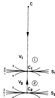
Fig. 6. Sketches of the cross-sections of the considered models in the plane of incidence E_{\parallel} : v_1 = 2,500 m/s; v_2 = 4,000 m/s; CC_1 = 1,500 m; C_1C_2 = 500 m; R_1^{(i)}(N) is the N -th version ( N = 0, 1, 2, 3, 4 ) of the principal radius of curvature of the interface S_i ( i=1, 2 ) in the plane E_1 = E_{\parallel} ; R_1^{(i)}(0) = \infty ; R_1^{(i)}(1) = 4,000 m; R_1^{(i)}(2) = -4,000 m; R_1^{(i)}(3) = 500 m; R_1^{(i)}(4) = -500 m
