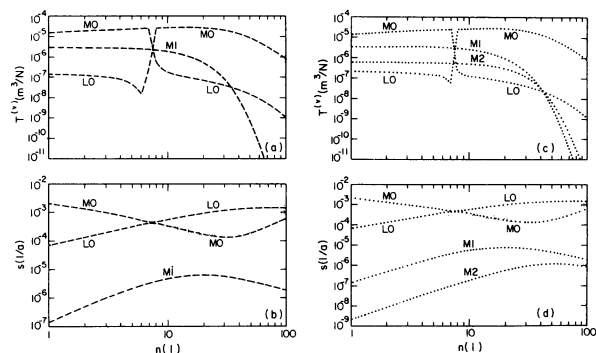
Fig. 8a–d. Same as Fig. 2 except for Earth Model M.2 (dashed) or Earth Model M.3 (dotted)
