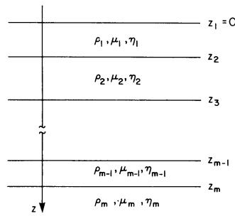
Fig. 1. Multi-layer Maxwell half-space
