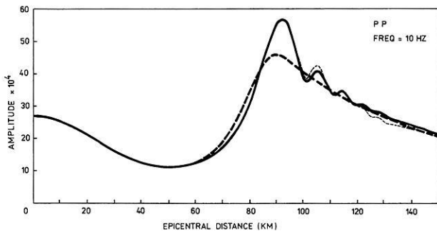
Fig. 8. Critical region. Amplitude-distance curves of PP refracted wave for the model shown in Fig. 6, computed by the summation of Gaussian beams. The Gaussian beam parameters are specified at the interface, K_0=0 \text{ km}^{-1} . The bold solid line corresponds to very broad Gaussian beams ( L_0=100 \text{ km} ) and the bold dashed line to very narrow Gaussian beams ( L_0=14 \text{ km} ). The thin dashed line corresponds again to narrow Gaussian beams ( L_0=14 \text{ km} ), with the exception of a very narrow vicinity of the critical point where L_0 increases smoothly from 14 km to 100 km at the critical point
