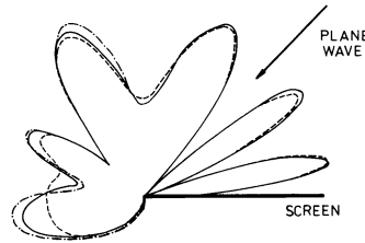
Fig. 10. The plane acoustic harmonic wave incident on a rigid half-screen. Propagation velocity in the model is 5 km/s, f=10 Hz, angle of incidence is 45^\circ . The parameters of Gaussian beams, chosen along the wavefront going through the edge, are K_0=0 km ^{-1} and L_0=1 km. The amplitudes of the complete wave field (incident+reflected) along a circle with its centre at the edgepoint and with a radius of 2\lambda ( =1 km) are shown. The bold line corresponds to the exact solution, the dashed line is obtained by the summation of Gaussian beams. The dot-dashed line also includes a diffracted wave generated at the edgepoint of the half-screen
