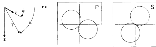
Fig. 17. Single-force radiation patterns. Left : The force is inclined by angle \varphi from the horizontal axis. Right : The single force radiation patterns of P and S waves for \varphi=30^\circ . The solid line denotes positive values, dashed line negative values. \vec{i} denotes the initial direction of the ray
