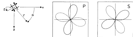
Fig. 18. Double couple radiation patterns. Left : Geometry of the source. Right : The double couple radiation patterns of P and S waves, \delta=30^\circ . The solid line denotes positive values, the dashed lines negative values. \vec{i} denotes the initial direction of the ray
