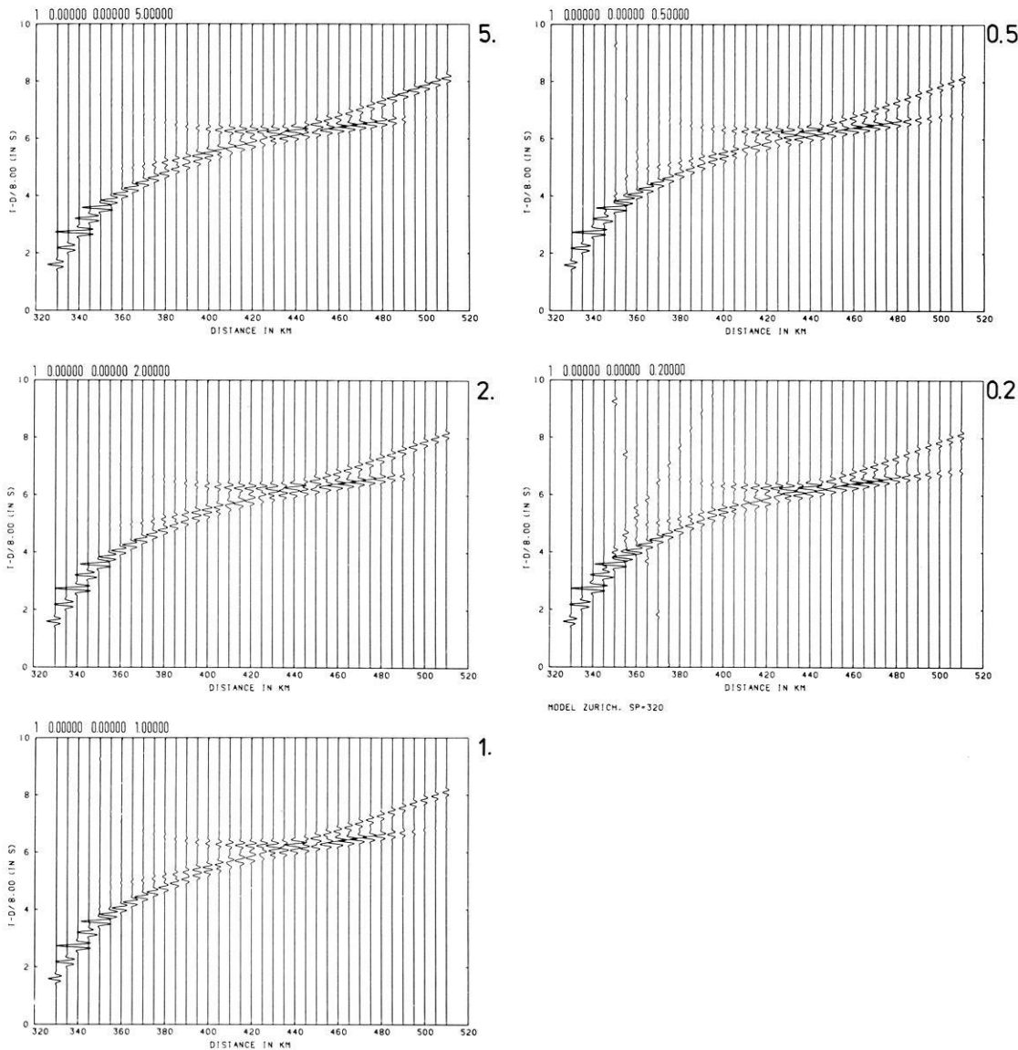
Fig. 14. Choice of parameters of Gaussian beams. Gaussian beam synthetic seismograms of the vertical component of the displacement vector in the model Zurich, SP=320 km (see Fig. 1). The parameters of Gaussian beams are chosen at the endpoints of rays, using Eq. (13) to determine \text{Re } M(O_s) and Eq. (15) to determine \text{Im } M(O_s) . Five seismogram sections for five different C , see Eq. (15), are shown: C=5, 2, 1, 0.5, 0.2 . The reduction velocity is 8 km/s
