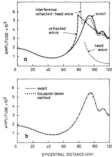
Fig. 7. Critical region. Top: Amplitude-distance curve of PP reflected wave in the model shown in Fig. 6, computed by the exact method (bold line), in comparison with ray computations. Bottom: the same, but in comparison with Gaussian beam computations (dots). The frequency is 6.4 Hz, Gaussian beam parameters chosen at the source are K_0 = 0 \text{ km}^{-1} , L_0 = 71.5 \text{ km}
