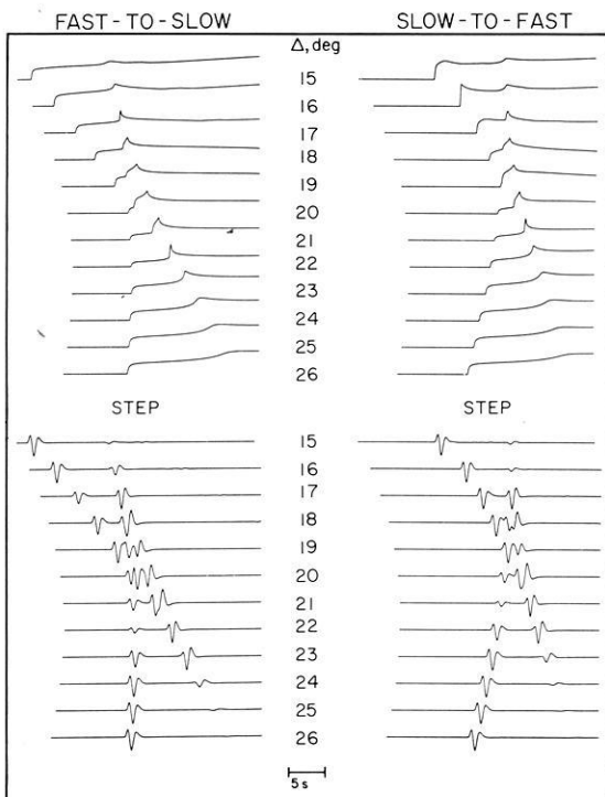
Fig. 13. Seismic sections plotted on the same reduced time scale. r = \Delta / (5.4 \text{ km/s}) . The synthetics are appropriate for a short-period WWSSN instrument response
