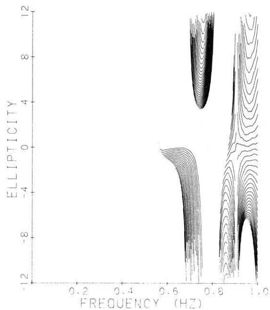
d) STRUCTURE: IMPI RAYLEIGH MODES 121 - 213
