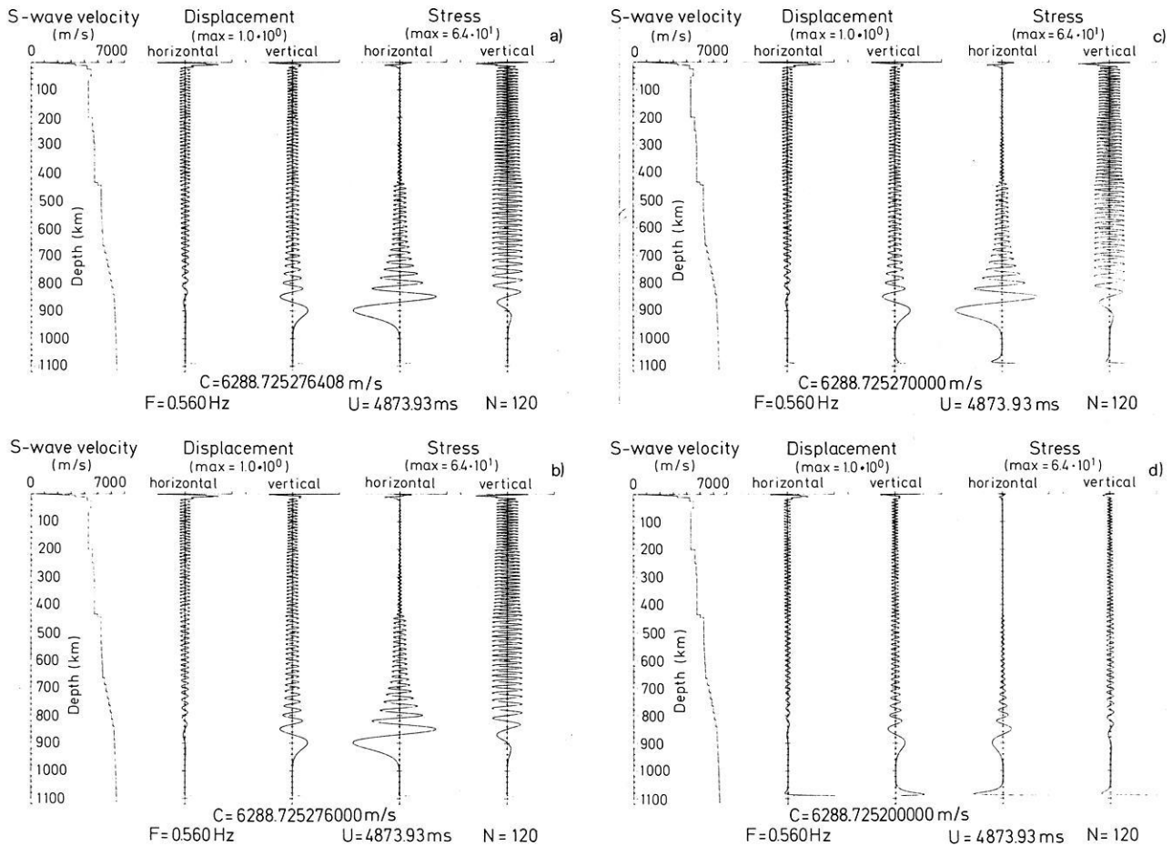
Fig. 8a-d. Example of the effect of truncating the precision of phase velocity in the determination of eigenfunctions for the higher mode number 120 at a frequency of 0.56 Hz for the continental structure: a phase velocity is determined with 13 figures; b phase velocity is determined with 10 figures; c phase velocity is determined with 9 figures; d phase velocity is determined with 8 figures. From the figure it is evident that nine-ten figures in phase velocity are necessary to ensure the correct computation of eigenfunctions
