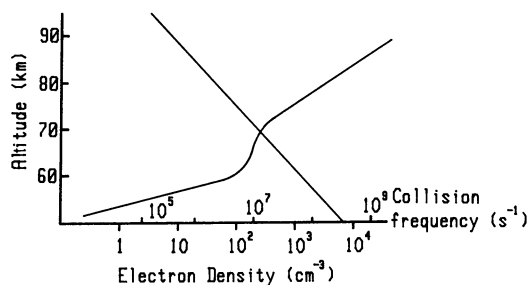
Fig. 7. Profiles of a typical daytime electron density and collision (electron-neutral) frequency, used in the calculation of the ionospheric transmission loss
