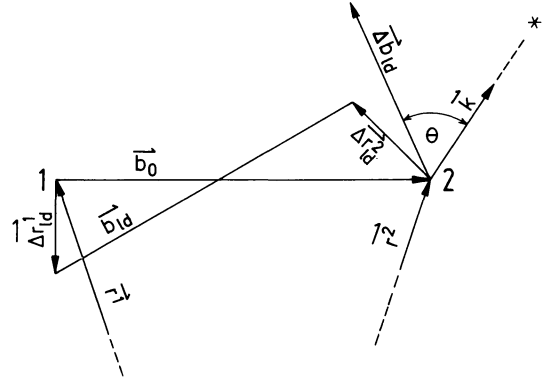
Fig. 3. Baseline-radiosource geometry of VLBI observations \vec{r}^i – position vectors of VLBI stations i=1,2 \vec{b}_0 – baseline vector under reference conditions \vec{b}_{id} – baseline vector after consideration of the load-induced displacements \Delta \vec{r}_{id}^i of the VLBI stations ( i=1,2 ) \Delta \vec{b}_{id} – load-induced baseline difference \vec{b}_{id} - \vec{b}_0 \vec{k} – unit vector in source direction \theta – angle between \Delta \vec{b}_{id} and \vec{k}
