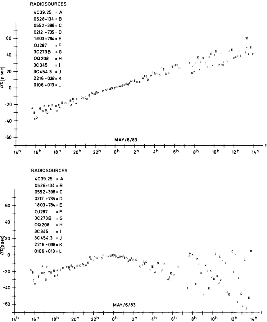
Fig. 5. Delay corrections \tau_{1d} caused by the station displacements simulated in Model 2 (see Fig. 4, top, left)
