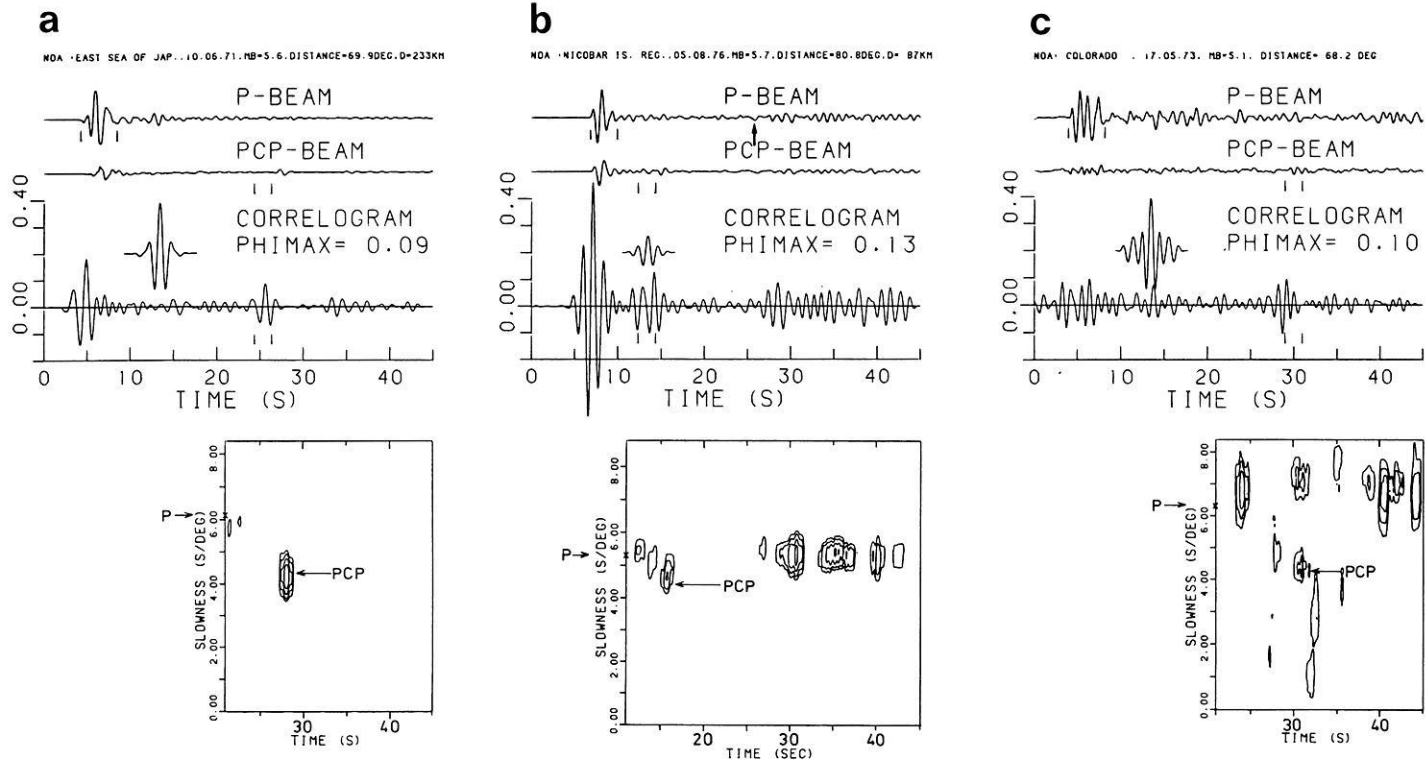
Fig. 2. a P , PcP beam, correlogram (upper part) and vespagram (lower part) for earthquake No. 10 from Table 1. The contour interval for the isolines in the vespagram is -3 dB. The arrows mark the slowness for P and PcP , respectively, after the Herrin tables. b The same as in Fig. 2a for earthquake No. 14 from Table 1. The arrow in the P beam marks the theoretical arrival time of the surface reflection pP . c The same as in Fig. 2a for the nuclear explosion in Colorado (No. 6 in Table 2)
