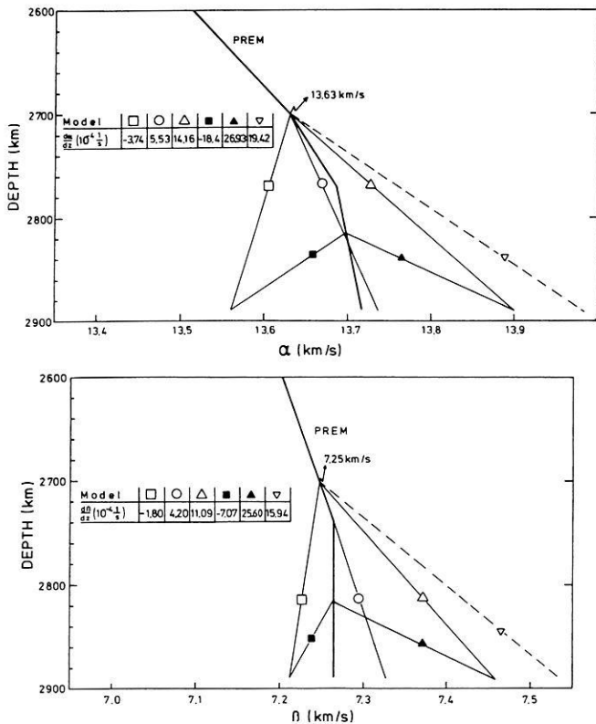
Fig. 8. P (above) and S velocity-depth function (below) for the low-velocity zone of the Earth's mantle with corresponding P - and S -velocity gradients \frac{d\alpha}{dz} and \frac{d\beta}{dz} . The heavy line corresponds to the PREM model of Dziewonski and Anderson (1981). The other models are named in the text as follows: □: N190, ○: M190, △: P190, ■: N75, ▲: P75, ▽: extreme, positive velocity gradient
