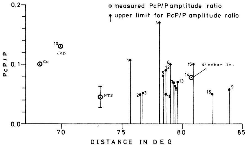
Fig. 7. PcP/P amplitude ratios for events with identifiable PcP signal ( \circ ) and upper limit for the PcP/P amplitude ratio for events without identifiable PcP signal ( \bullet ) for the earthquakes from Table 1 (with corresponding numbering) and for the nuclear explosions from Table 2. The value marked 'NTS' corresponds to the mean value (with bars indicating standard deviations) of all PHIMAX values from the nuclear explosions from the Nevada Test Site. 'Co' corresponds to the value for the nuclear explosion in Colorado (No. 6 in Table 2). All earthquake data have been corrected for isotropic source radiation
