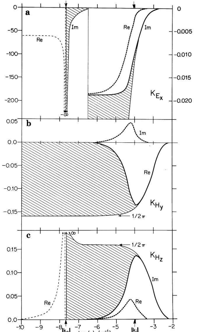
Fig. 2a–c. The bold lines illustrate the kernels for a line current at a depth of 1 km in a half-space of 1,000 \Omega\text{m} excited at a frequency of 1 Hz, whereas the light lines are those for a line current in free space. The shaded regions are those areas included in the integral when the line current is considered to be in free space. a K_{E_x}(v) , (Im in full lines, Re in dashed) – note the dramatic change in ordinate scale at v = 10|k_0| , b K_{H_y}(v) , (Re in full lines, Im in dashed), c K_{H_z}(v) , (Im in full lines, Re in dashed)
