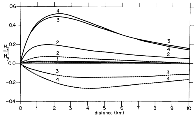
Fig. 6. The ratio of the vertical magnetic field to the total horizontal magnetic field, for the model illustrated in Fig. 5 at a frequency of 1 Hz for the four different block resistivities. \text{Re}[H_z(y)/H'_y(y)] in full line, \text{Im}[H_z(y)/H'_y(y)] dashed line
