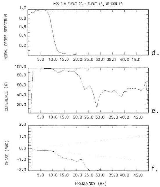
Fig. 8a-f. Cross spectral analysis of the E-W component seismograms for event 16 as compared with event 20. Recording site is MSS. For explanations, see Figs. 3 and 4
