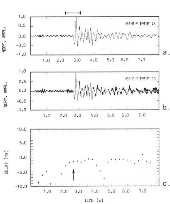
Fig. 8a-f. Cross spectral analysis of the E-W component seismograms for event 16 as compared with event 20. Recording site is MSS. For explanations, see Figs. 3 and 4
