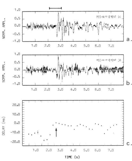
Fig. 7a-f. Cross spectral analysis of the N-S component seismograms for event 16 as compared with event 20. Recording site is MSS. For explanations, see Figs. 3 and 4
