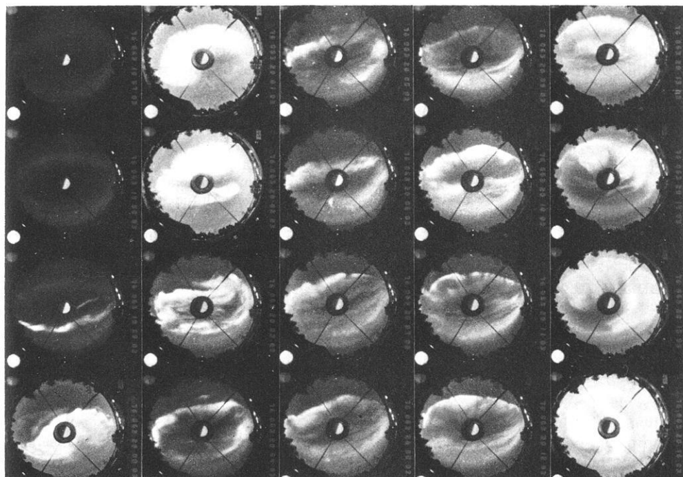
Fig. 5. All-sky camera data recorded at Muonio from 1957 to 2016 UT
