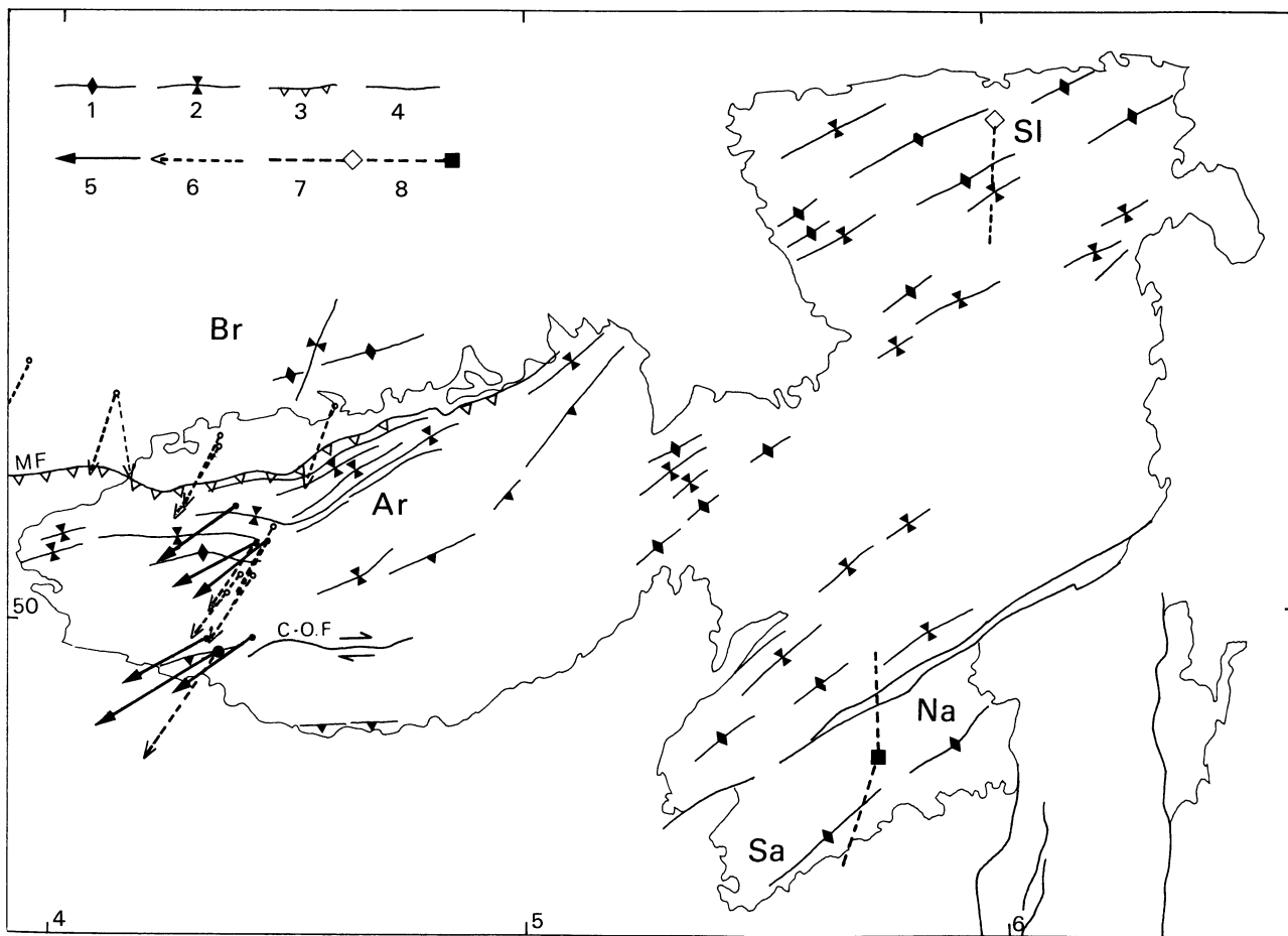
Fig. 5. Tectonic sketch map and paleomagnetic results of the Ardenne and the Rhenish massif. 1: anticline axis; 2: syncline axis; 3: thrust fault; 4: fault; 5: Westphalian–Stephanian B overprint directions; 6: Stephanian–Permian A overprint directions; 7: mean direction of remagnetization in the Sauerland (S1) (Bachtadse, 1983); 8: mean directions in Permian volcanics of the Saar-Nahe (Sa-Na) (Nijenhuis, 1961; Berthold et al., 1975); MF: Midi fault; C-O.F.: La Carbonnière-Opont strike-slip fault
