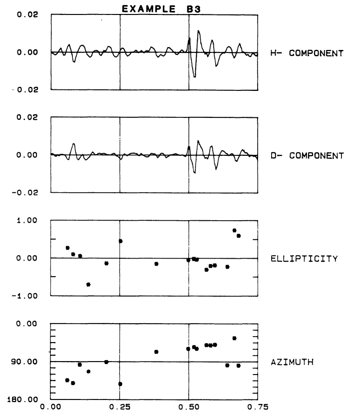
Fig. 3a-c. Three examples of the time-domain polarization analysis of background sferics. H and D correspond to the N-S and E-W magnetic components. a example B1; b example B2; c example B3
