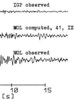
Fig. 8. The same as Fig. 6, but for receiver IX of profile 4 and model 41. Model 41 is the two-layered basin. Again, the middle trace was obtained from the top one, without any knowledge of the bottom “target” trace. For other examples with different models and profiles, see Zahradník and Hron (1986)
