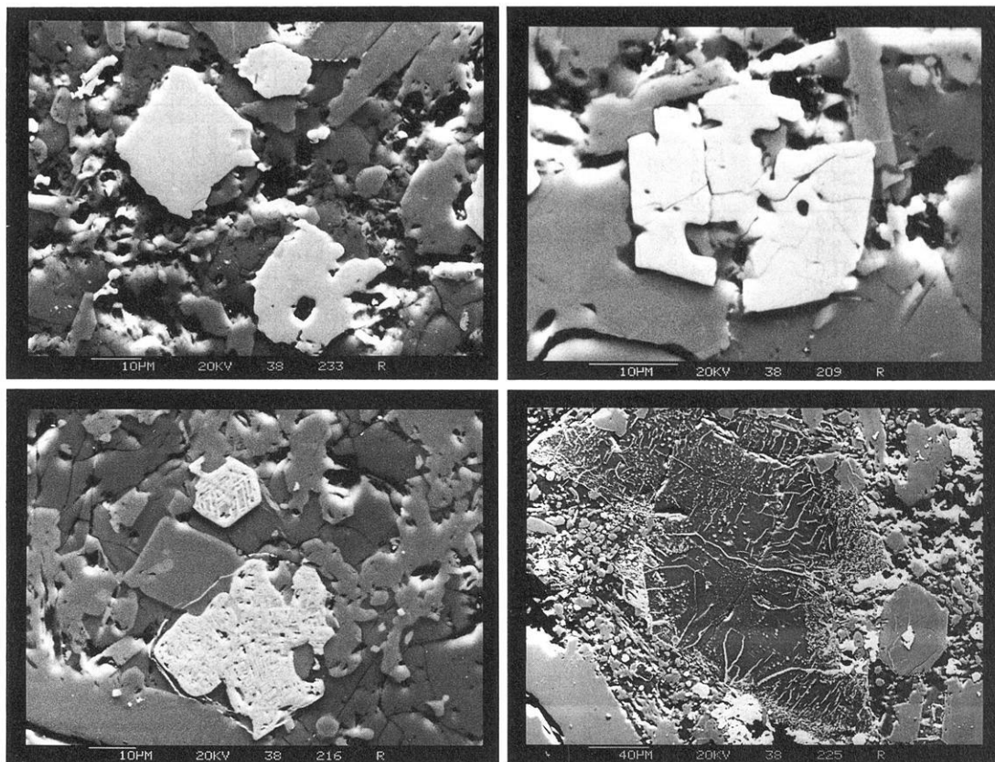
Fig. 2a–d. Examples for SEM studies on polished sections. a partly anhedral titanomagnetites, typical for many specimens; b maghemitized titanomagnetite; c strongly oxidized titanomagnetite; d hematite skeleton as alteration product of olivine
