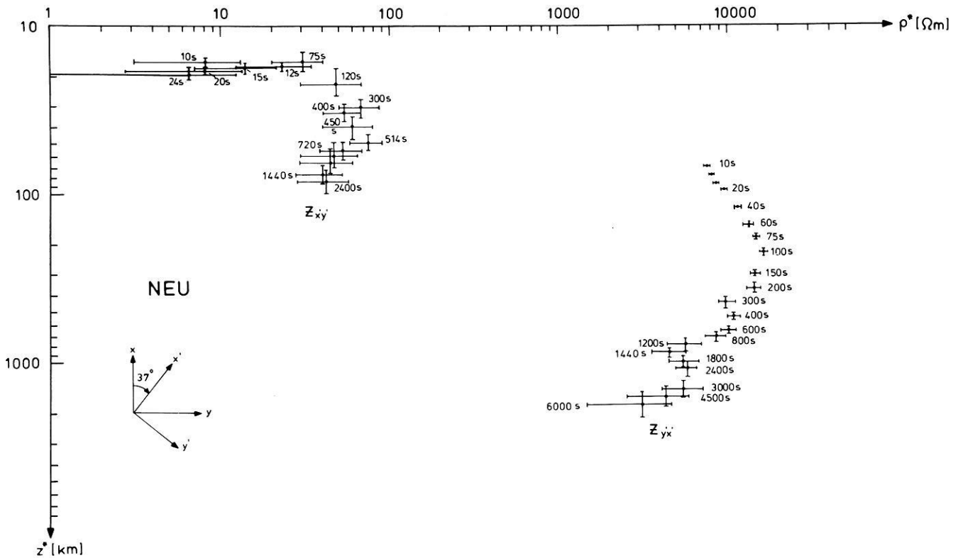
Fig. 7. \rho^*(z^*) curves of E -( Z_{x'y'} )- and B -( Z_{yx'} )-polarisation for the Schwarzwald station NEU. Only the \rho^*(z^*) curve for E -polarisation should be considered as a representation of the true conductivity distribution beneath the Schwarzwald. Note that z^* values concentrate at 20 km with apparent resistivities below 10 \Omega\text{m} between 10 and 75 s, reflecting the top of the crustal conductor beneath crystalline. Observe the ascent in \rho^* below that depth, indicating a transition to a normal mantle resistivity of 50 \Omega\text{m}
